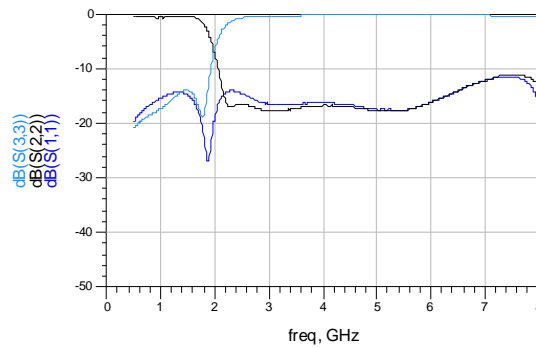
Return Loss
